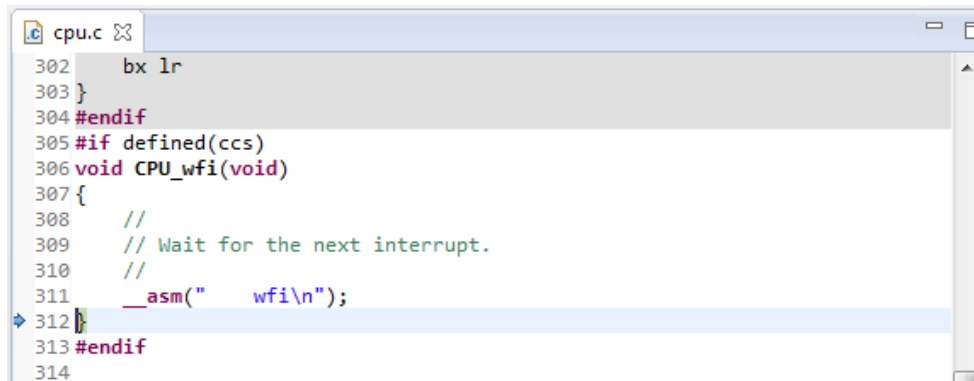
Figure 46. Program Counter Located at WFI Instruction
