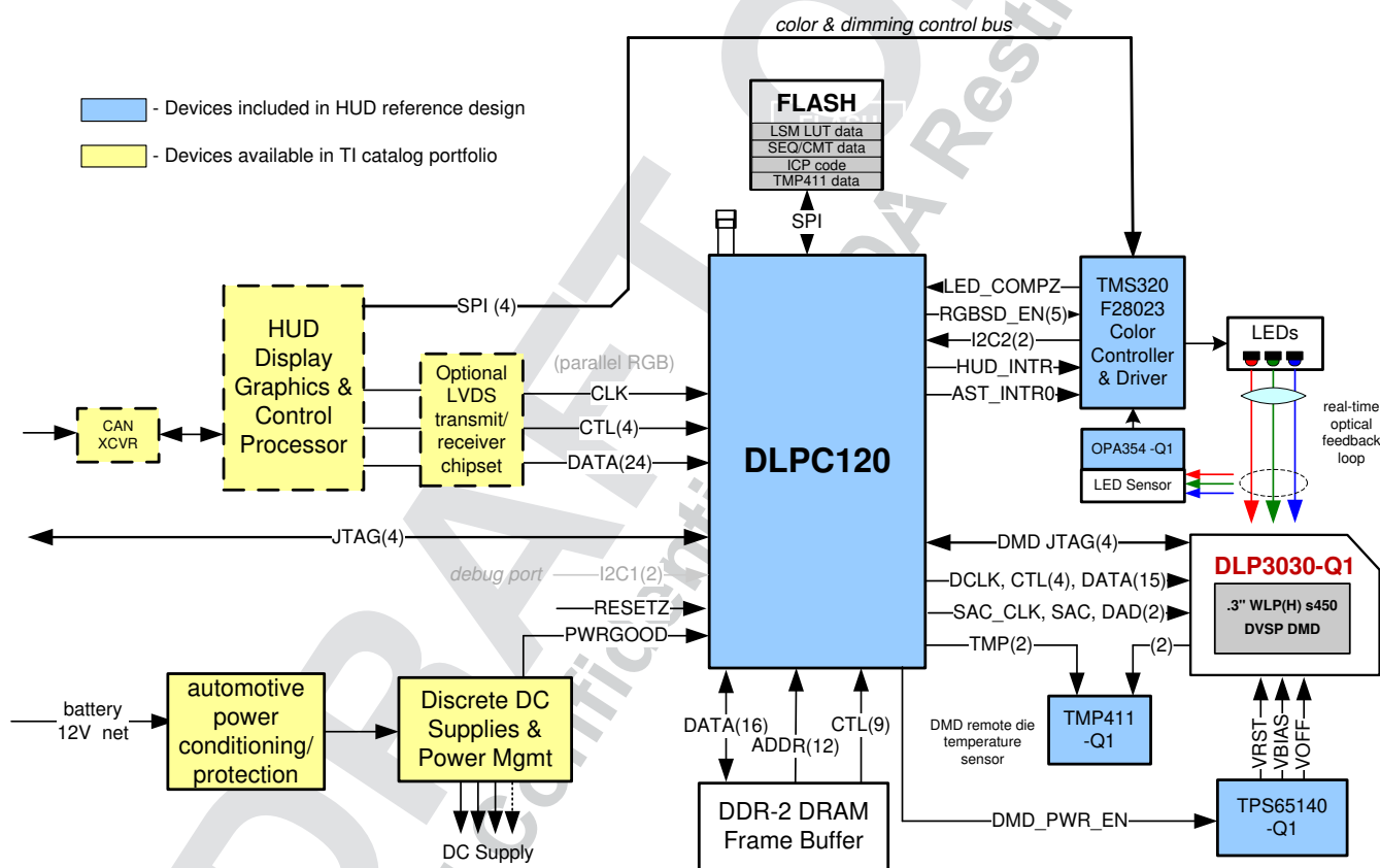
Figure 1-1. Piccolo LED Controller Block Diagram
