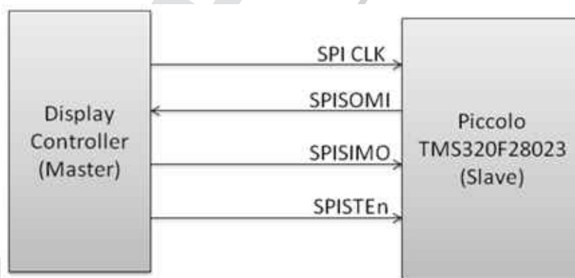
Figure 1-1. Block Diagram
