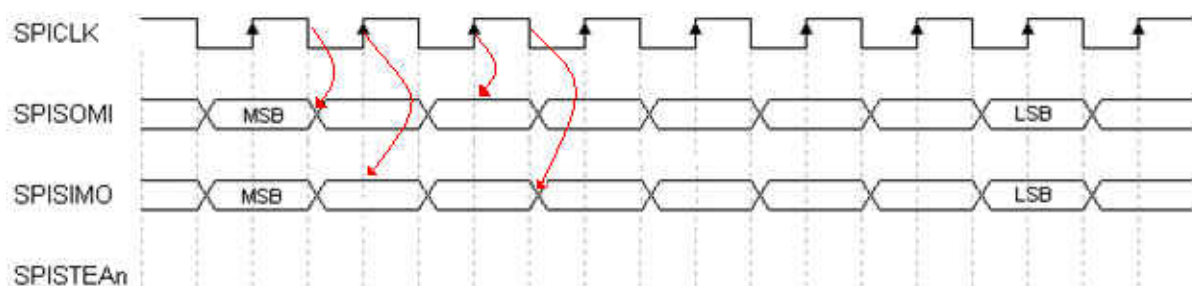
Figure 1-2. Signal Format
