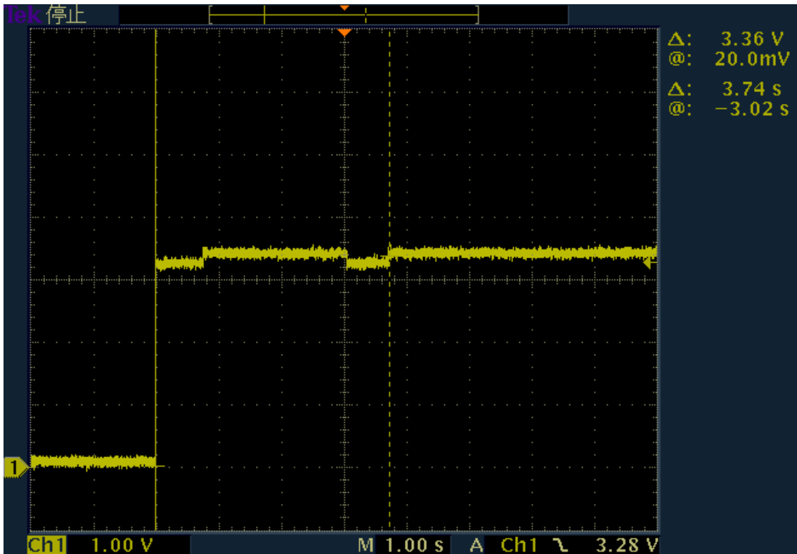
Measured waveform
