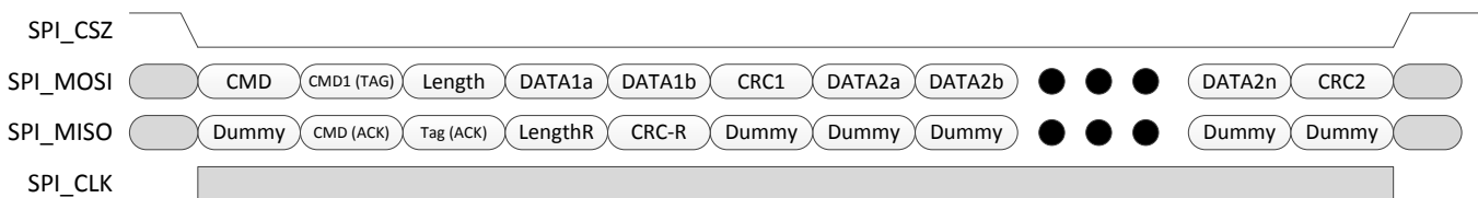
Figure 3-3. SPI Bulk Write
