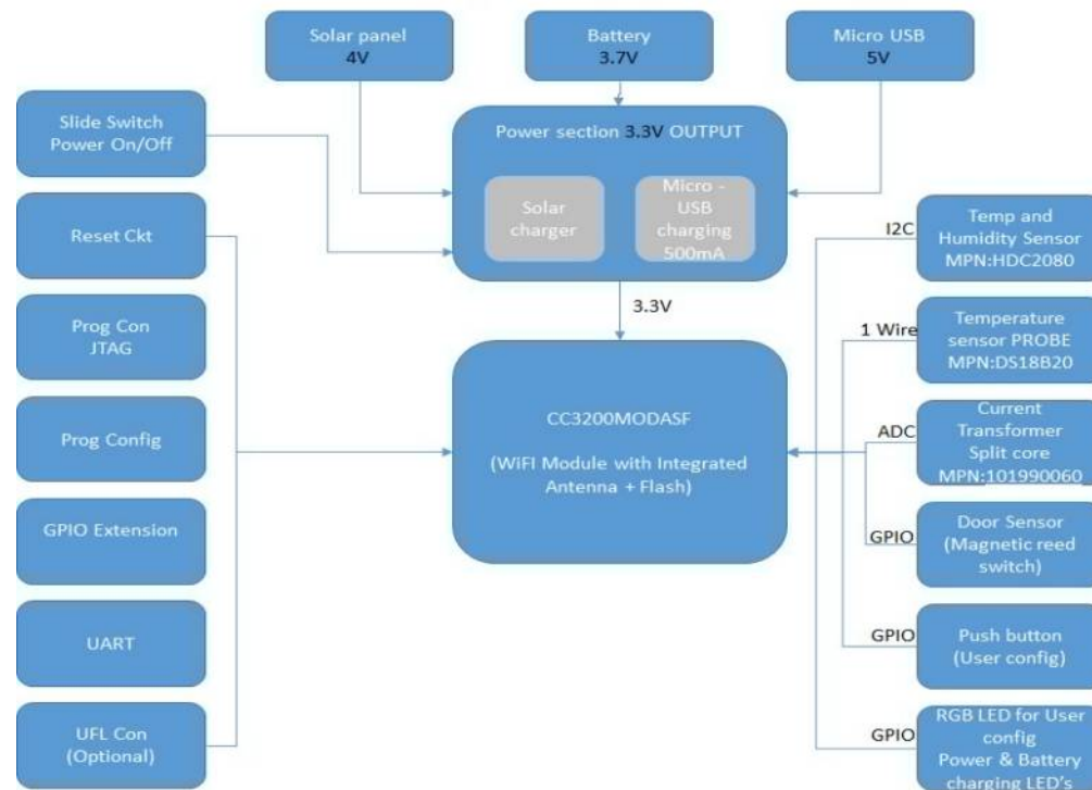
Block Diagram Of Equipment Monitoring
