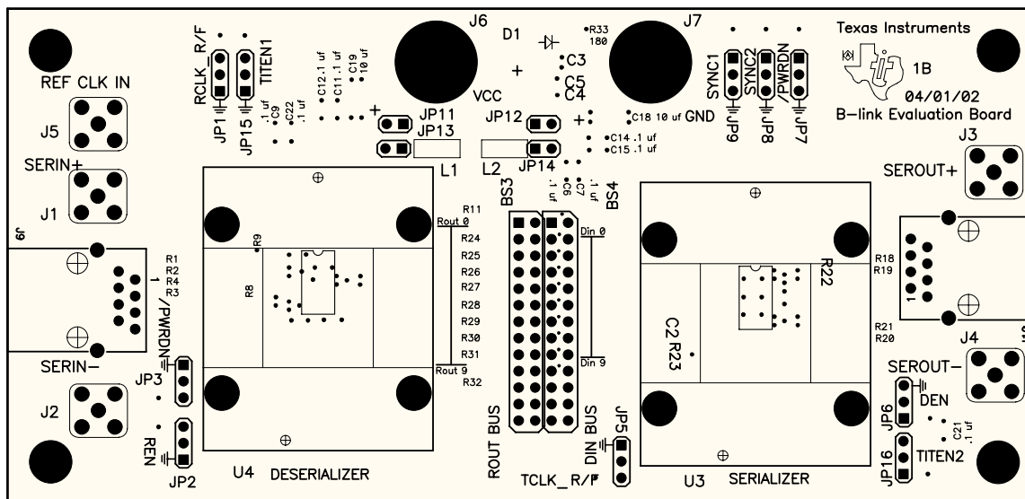
Top Silkscreen
