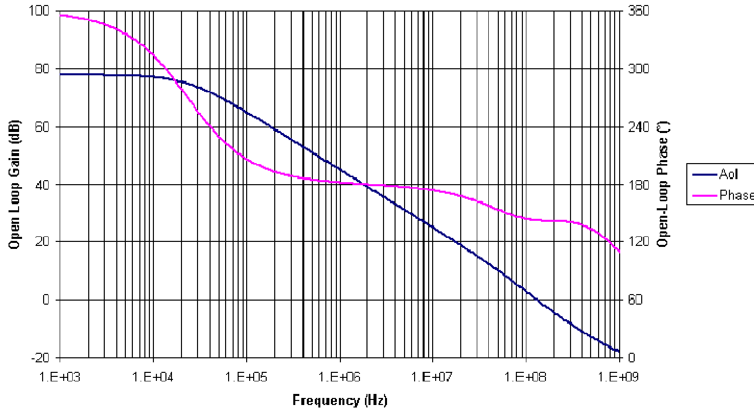
THS4130 Open Loop Gain and Phase
