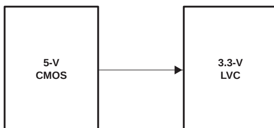
Case 3: 5-V CMOS Device Driving 3.3-V TTL Device (LVC)
