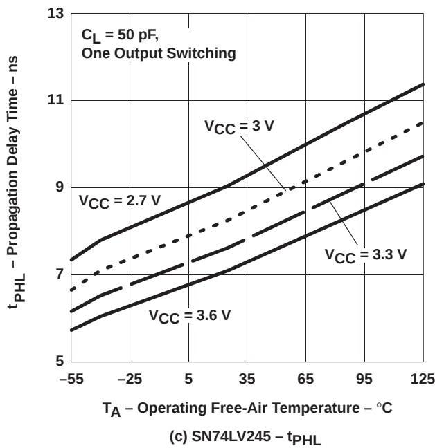
Figure 3. Propagation Delay Time Versus Operating Free-Air Temperature
