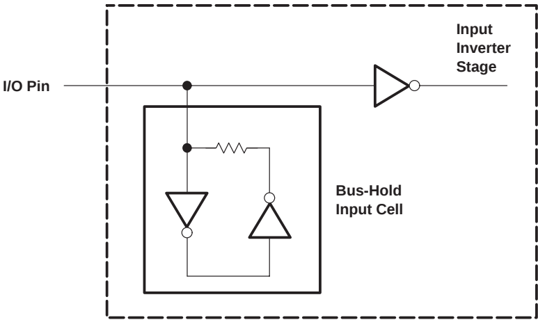
Figure 12. Bus Hold
