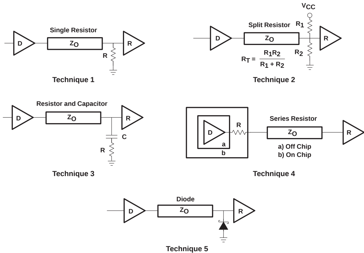
Figure 16. Termination Techniques
