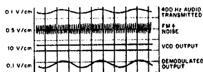
Fig. 11— Voltage waveforms of FM demodulator.
