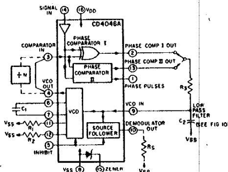
Fig. 2- COS/MOS PLL block diagram.
