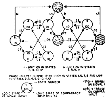
Fig. 7 -- State diagram of phase-comparator II.
