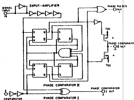
Fig. 3- Schematic of COS/MOS PLL phase-comparator section.
