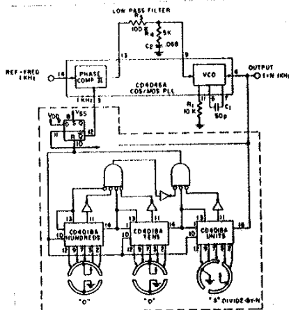
Fig. 12— Low-frequency synthesizer with three-decade programmable divider.
