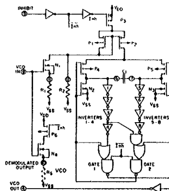
Fig. 8 -- Schematic of COS/MOS VCO section.
