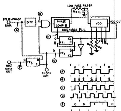
Fig. 14— Split-phase data synchronization and decoding.
