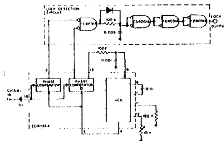
Fig. 15— Lock-detection circuit.
