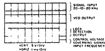
Fig. 16— Lock-detection-circuit waveforms.
