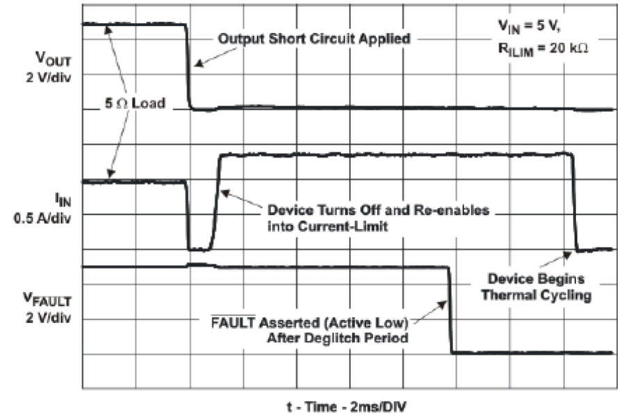
Figure 9. Full-Load to Short-Circuit Transient Response
