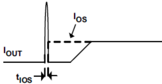
Figure 3. Response Time to Short Circuit Waveform
