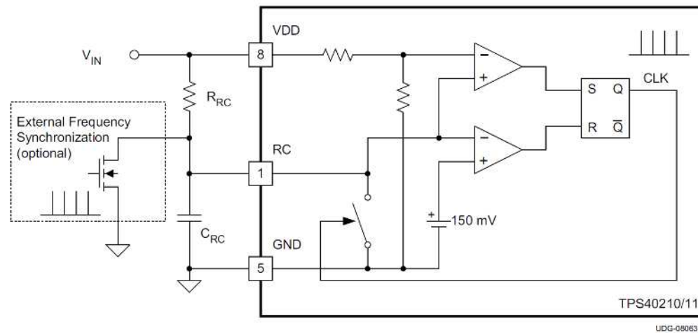
Figure 20. Oscillator Functional Diagram
