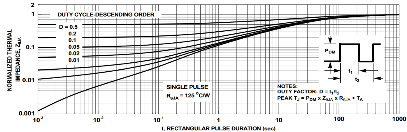
Figure 1. Transient Thermal Impedance
