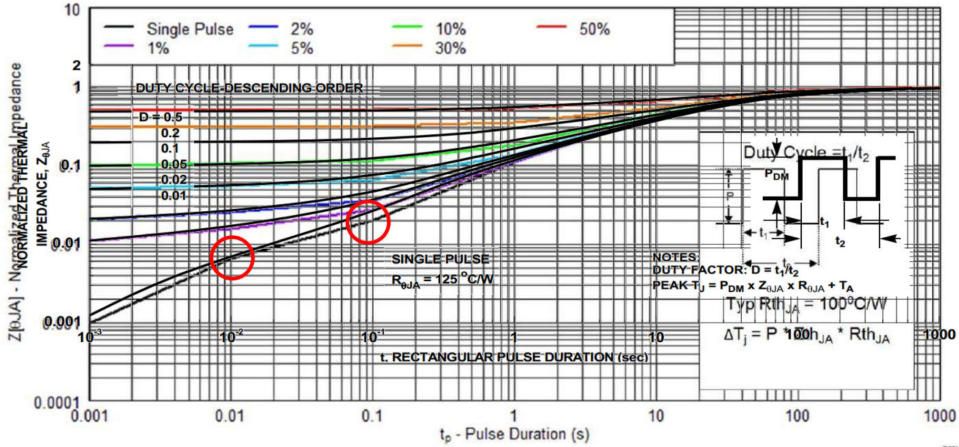
Figure 1. Transient Thermal Impedance
