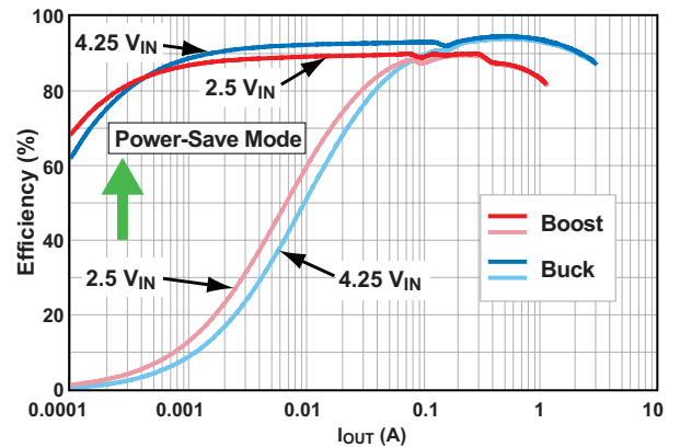
TPS63020 efficiency at 3.3 V.
