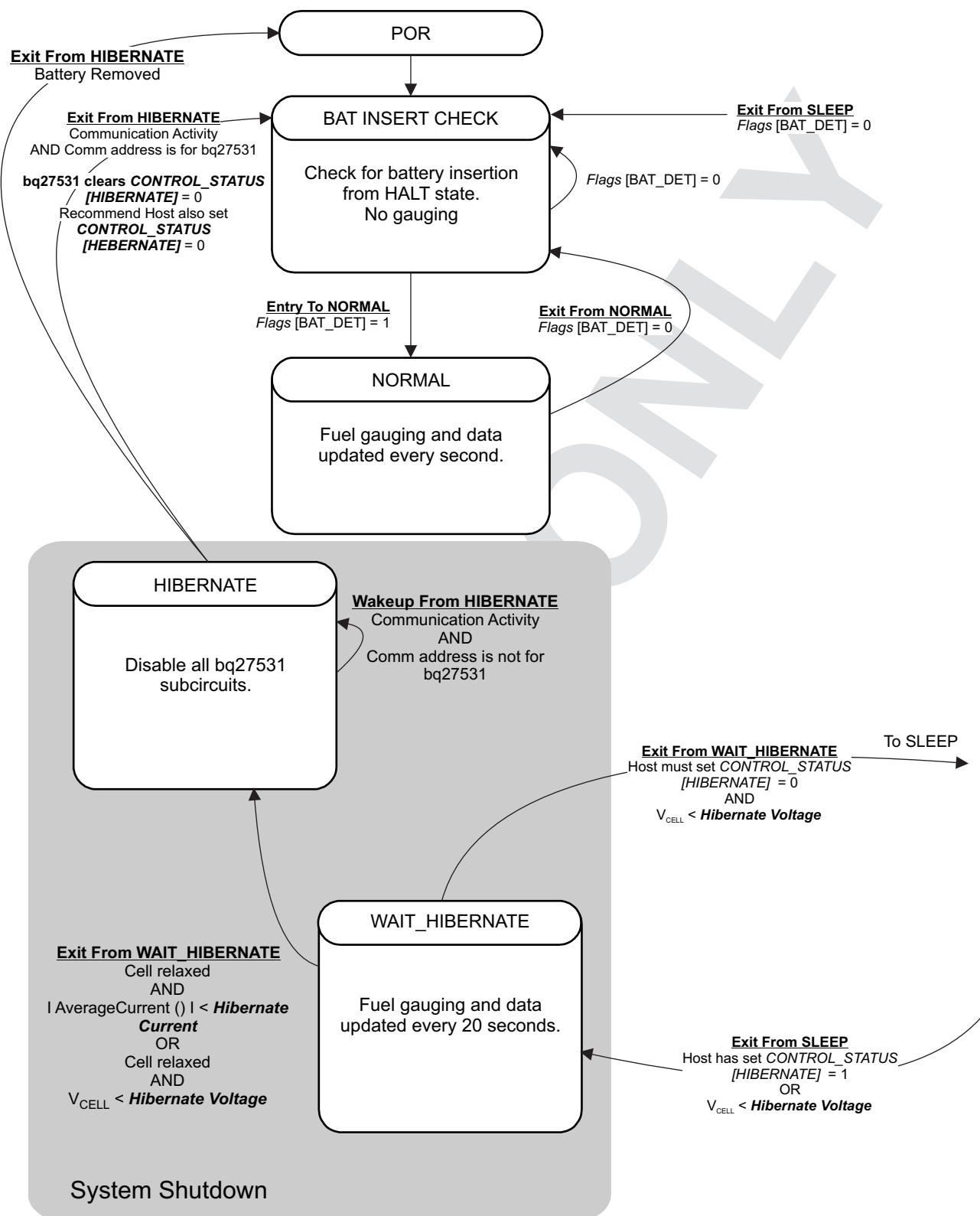
Figure 6-2. Power Mode Diagram—System Shutdown
