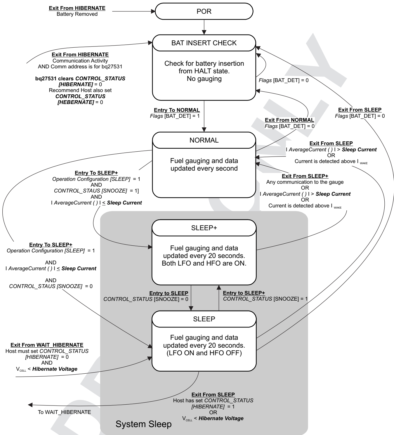
Figure 6-1. Power Mode Diagram—System Sleep
