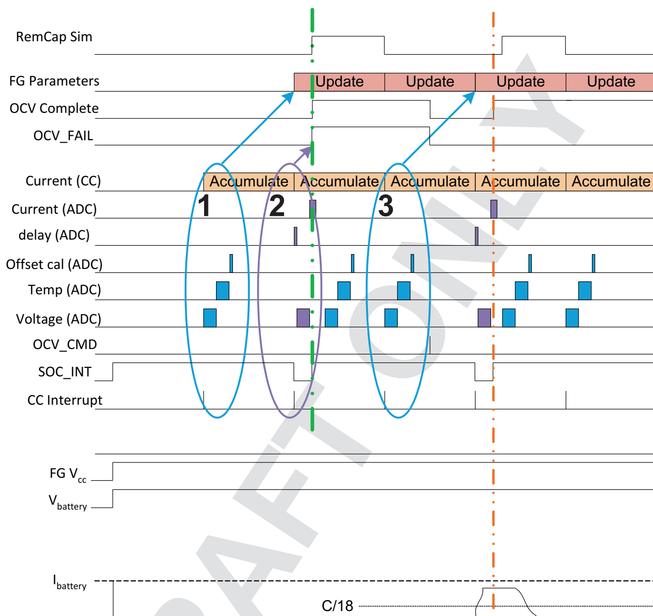
Figure A-1. OCV Timing Sequences
