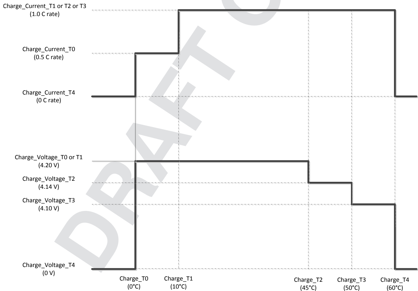
Figure 3-2. Charging Profile Based on Temperature Range
