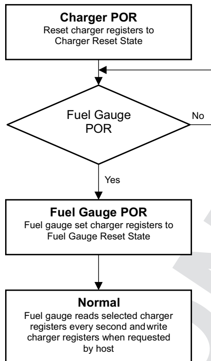
Figure 3-1. Charger Power-up
