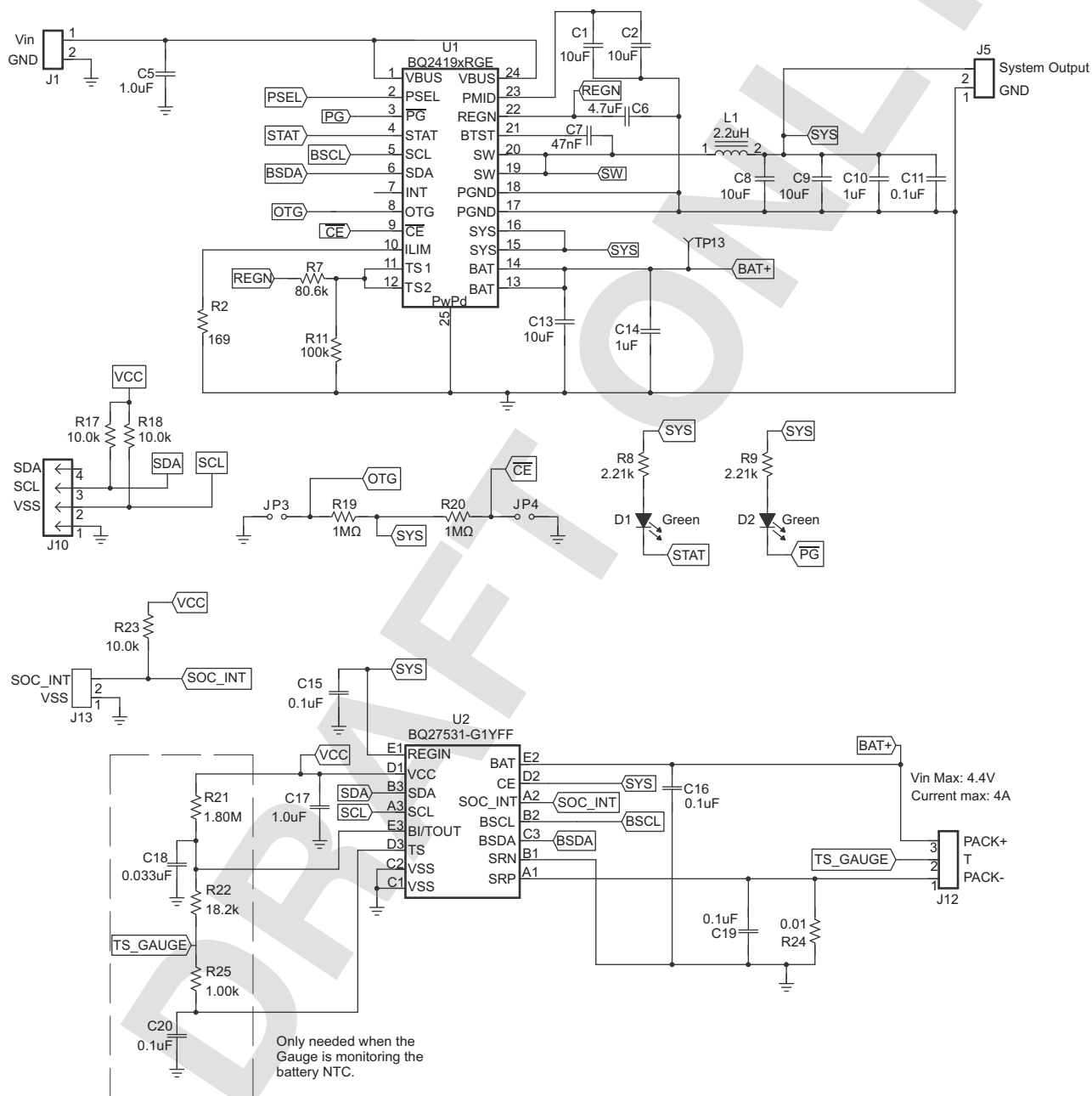
Figure 9-1. Charger Application Schematic
