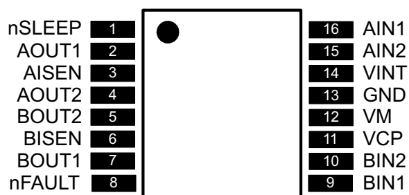
PW PACKAGE (TOP VIEW)
