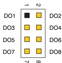
Figure 1. Connector J2
