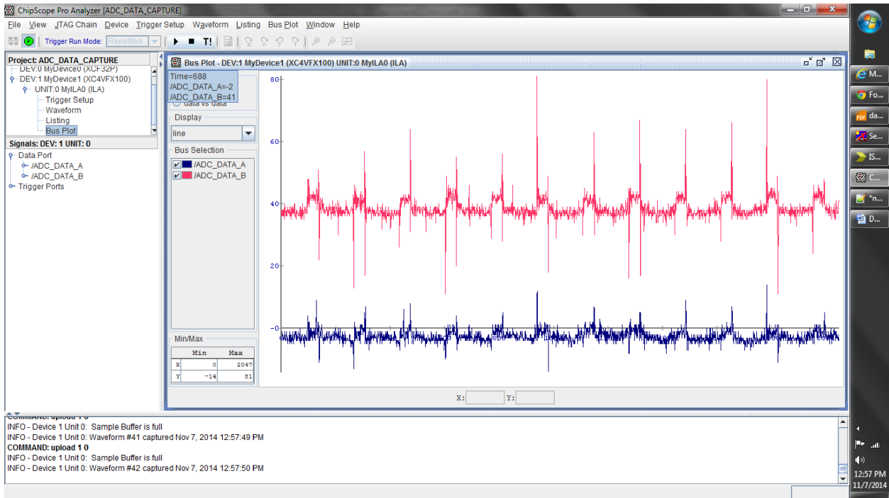
Waveform of each channel when terminated with 50 ohm
