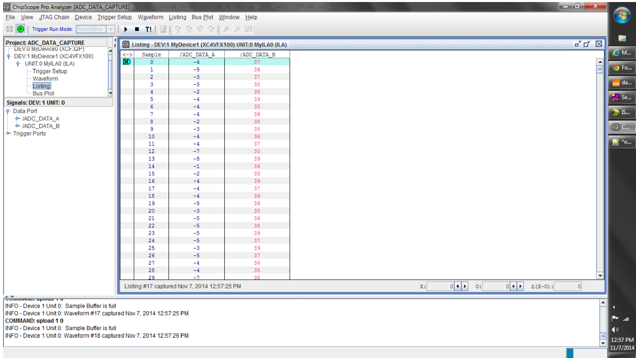
Data Values of each channel when terminated with 50ohms
