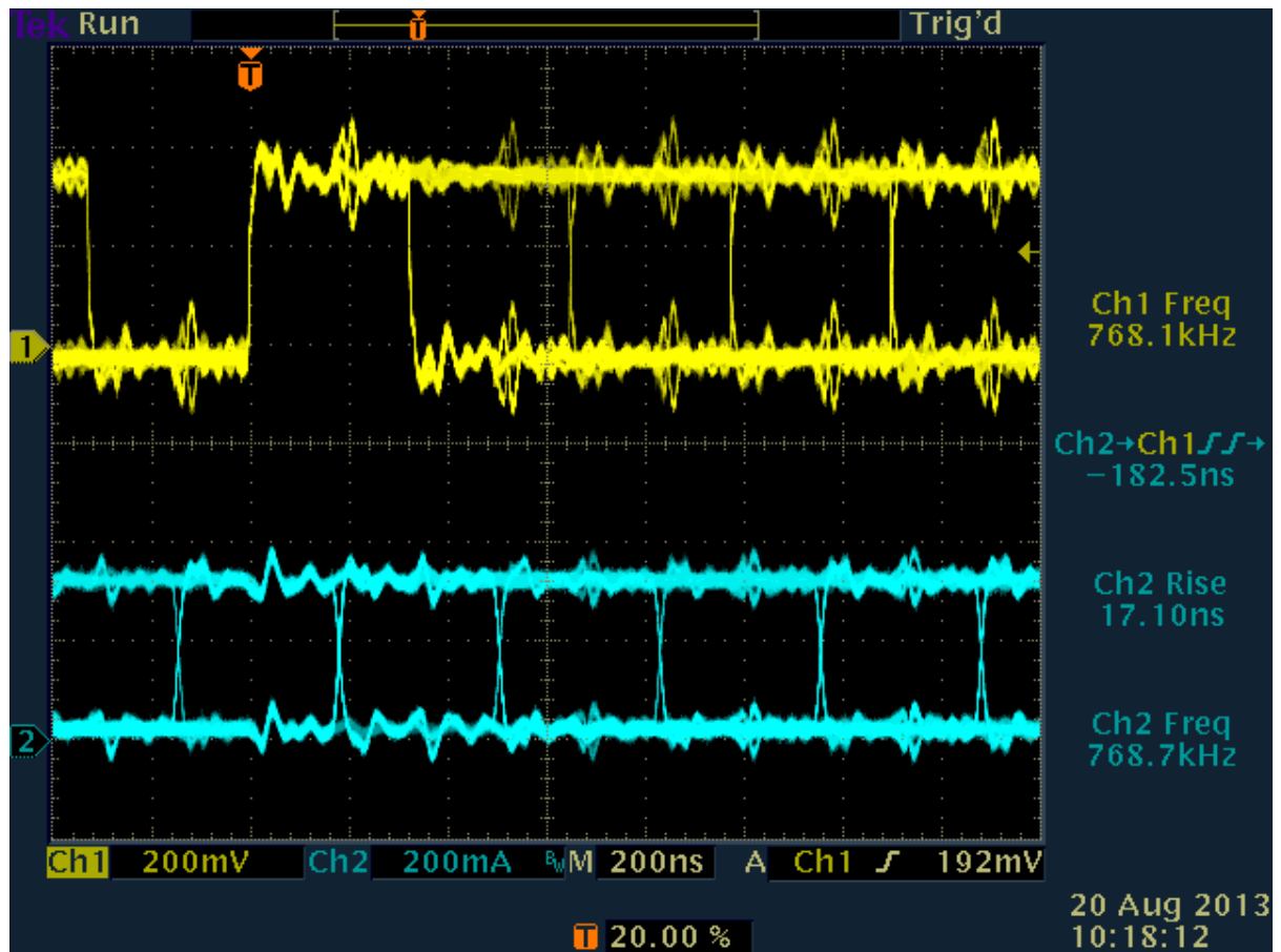
Codec Data In (Y) and Data Out (B)
