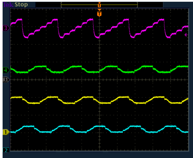
Fig. 19 (a) mod6 counter, (b)BemfA, (c) BemfB (c)BemfC (under 0.5 pu load at 0.3pu speed, Vdcbus=160V)
