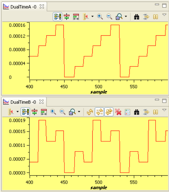
Fig. 15 (a) mod6 counter, (b) HallGpioAccepted (dlog.prescalar=25 and Vdcbus=160V)
